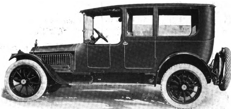
Limousine body on Packard chassis. Note the pleasing effect of the special streamline cover.
